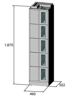
Locker Slim puerta M
