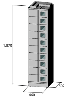
Locker Slim puerta S
